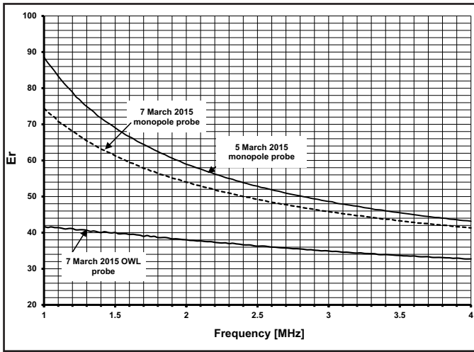
Figure 23 — Soil relative permittivity measurements.
