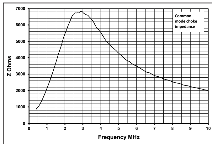
Figure 5 — Measured impedance of the common mode choke.
