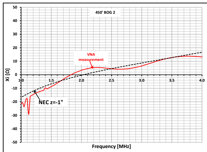
Figure 37 — Measured and computed BOG reactance.
