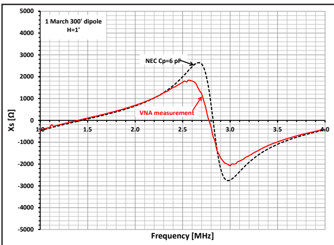
Figure 11 — Reactance measurement at antenna height of 12 inches.
