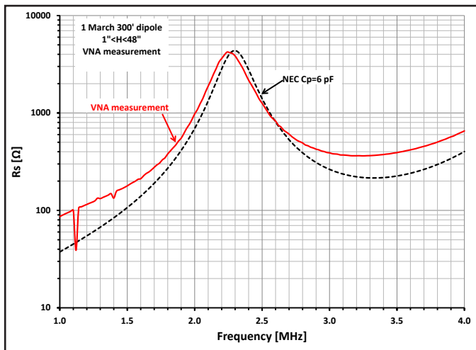
Figure 16 — Resistance measurement at antenna height of 1 inches.
