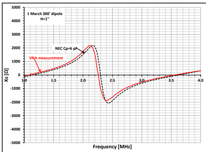
Figure 17 — Reactance measurement at antenna height of 1 inches.
