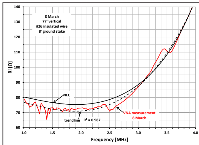
Figure 30 — Measured and computed resistance of the 77 foot vertical with a single ground stake.
