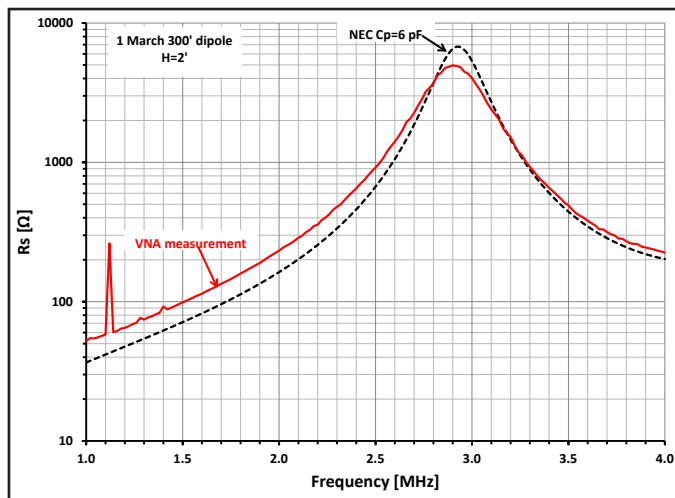
Figure 8 — Resistance measurement at antenna height of 24 inches.
