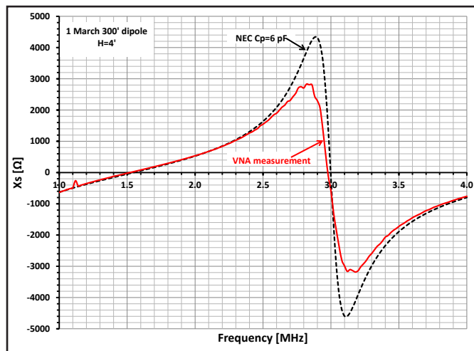
Figure 7 — Reactance measurement at antenna height of 48 inches.
