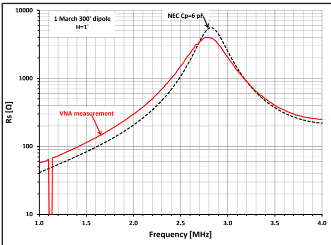
Figure 10 — Resistance measurement at antenna height of 12 inches.
