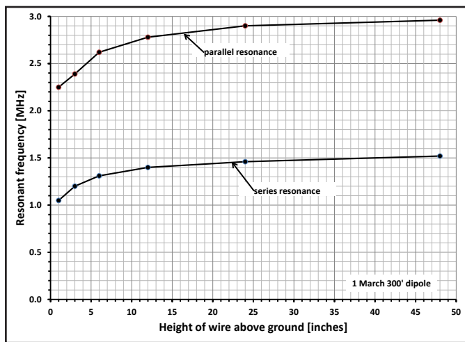
Figure 18 — Resonance variation with height for the 300 foot dipole.
