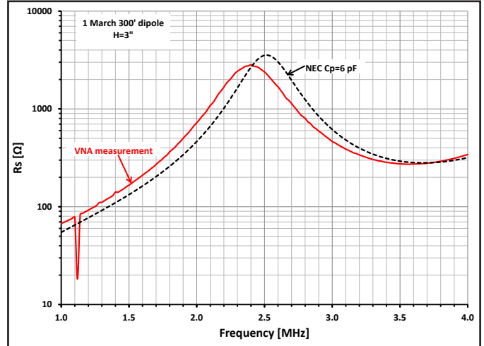
Figure 14 — Resistance measurement at antenna height of 3 inches.
