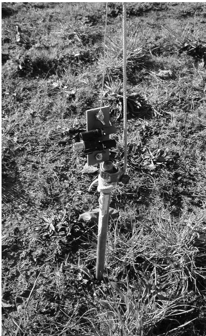
Figure 29 — Feed point and ground rod of test antenna #3.
