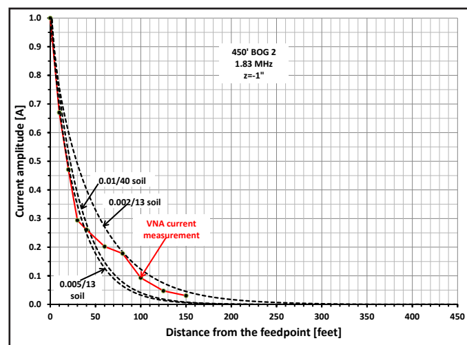
Figure 38 — Measured and computed BOG current amplitude.
