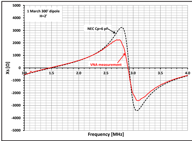
Figure 9 — Reactance measurement at antenna height of 24 inches.
