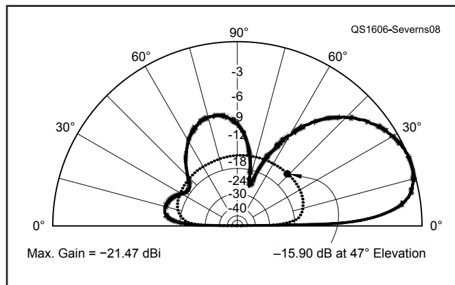
Figure 39 — Computed elevation antenna patterns for the BOG one inch above and one inch below ground.
