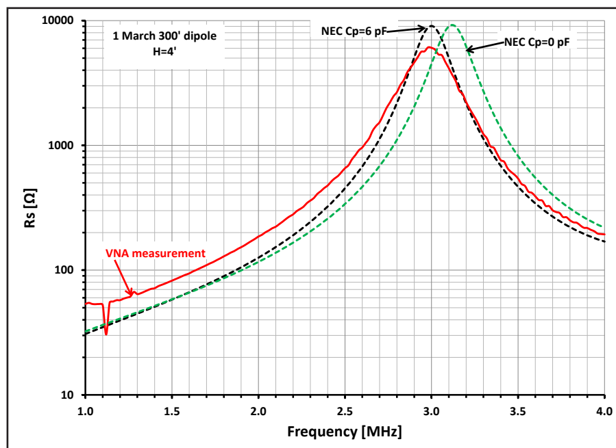
Figure 4 — Modeling with and without C_p .
