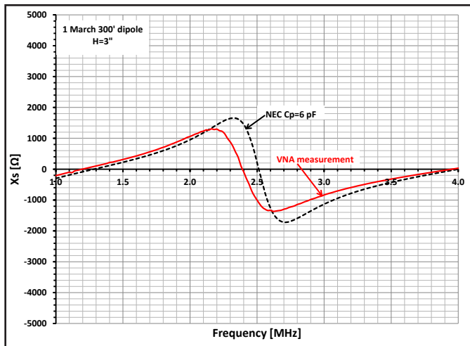
Figure 15 — Reactance measurement at antenna height of 3 inches.
