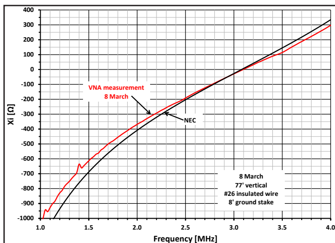
Figure 31 — Measured and computed reactance of the 77 foot vertical with a single ground stake.
