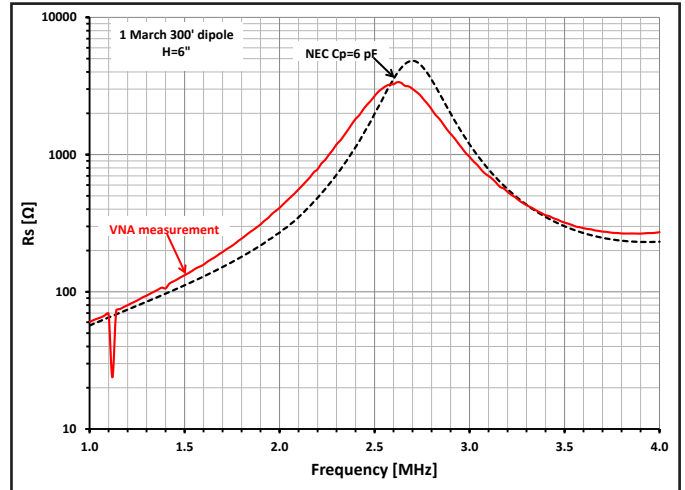
Figure 12 — Resistance measurement at antenna height of 6 inches.
