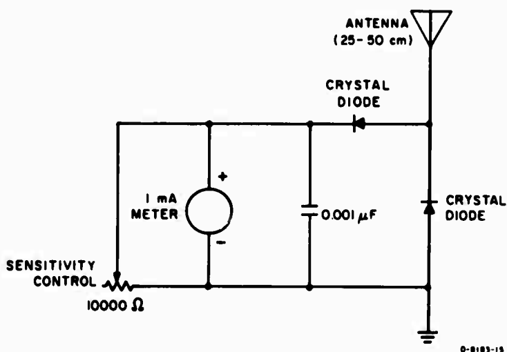
FIG. A-3 FIELD STRENGTH INDICATOR
