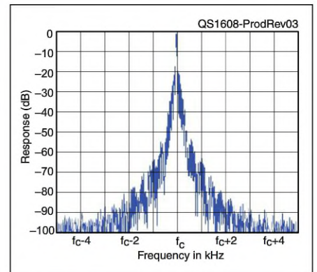
Figure 3 — Spectral display of the Icom IC-7300 transmitter during keying sideband testing. Equivalent keying speed is 60 WPM using external keying. Spectrum analyzer resolution bandwidth is 10 Hz, and the sweep time is 30 seconds. The transmitter was being operated at 100 W PEP output on the 14 MHz band, and this plot shows the transmitter output ±5 kHz from the carrier. The reference level is 0 dBc, and the vertical scale is 10 dB/division.
