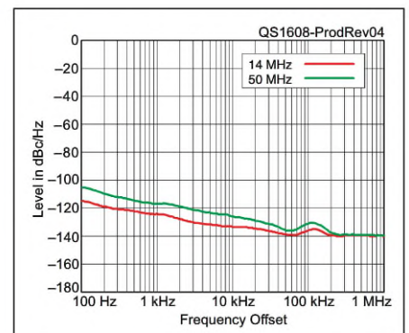
Figure 4 — Spectral display of the Icom IC-7300 transmitter output during phase noise testing. Power output is 100 W on the 14 MHz band (red trace) and 50 MHz band (green trace). The carrier, off the left edge of the plot, is not shown. This plot shows composite transmitted noise 100 Hz to 1 MHz from the carrier. The reference level is 0 dBc, and the vertical scale is in dBc/Hz.
