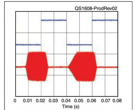
Figure 2 — CW keying waveform for the Icom IC-7300 showing the first two dits using external keying. Equivalent keying speed is 60 WPM. The upper trace is the actual key closure; the lower trace is the RF envelope. (Note that the first key closure starts at the left edge of the figure.) Horizontal divisions are 10 ms. The transceiver was being operated at 100 W output on the 14 MHz band.
