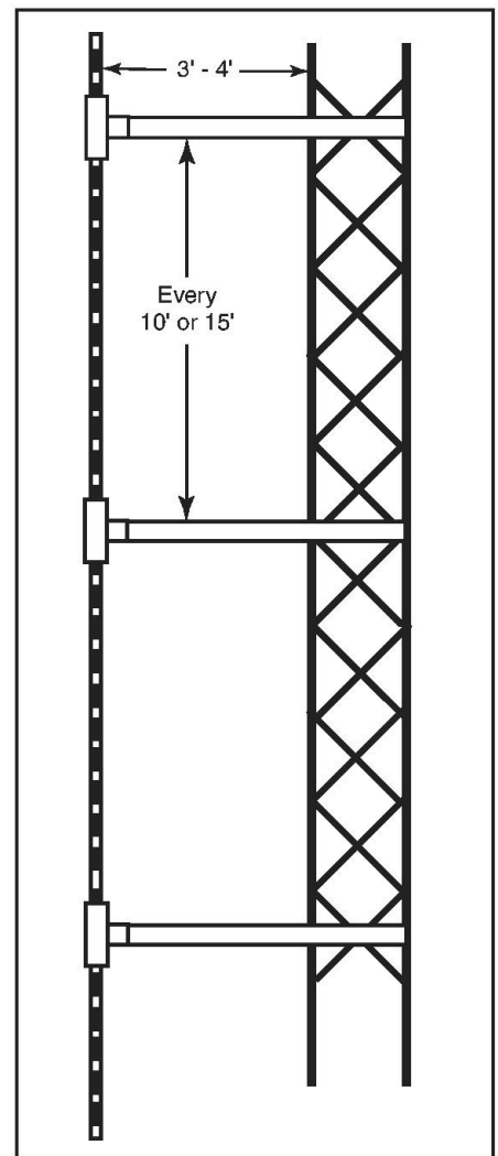
Figure 7— The 450 Ω ladder line runs through 3/4 inch PVC standoffs spaced down the tower. Attach the feed line to the standoffs with cable ties.
