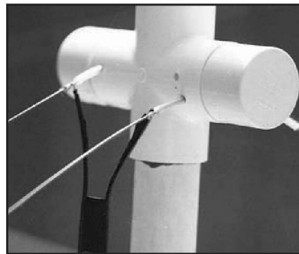
Figure 4—A PVC T or 4-way adapter supports two element crossover wires above the boom and provides a convenient attachment point for the 450 Ω feed line. The crossover wires are made from no. 12 Copperweld wire and double as guy wires for the twin boom.
