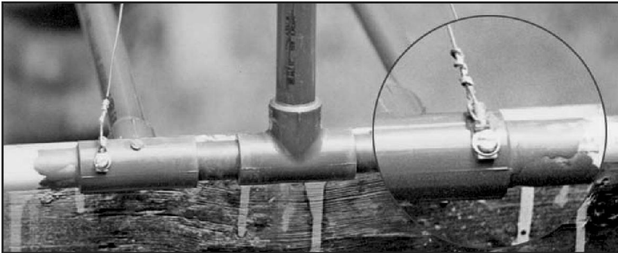
Figure 5— The crossover feed wires are attached to the element ends with large solder lugs and stainless sheet metal screws. Weatherproof the connection with a blob of silicone sealant.
